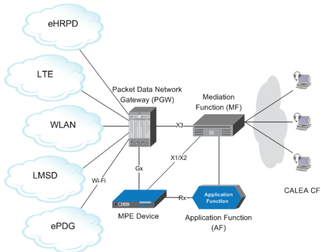
Figure 1-1 Lawful Intercept Architecture
